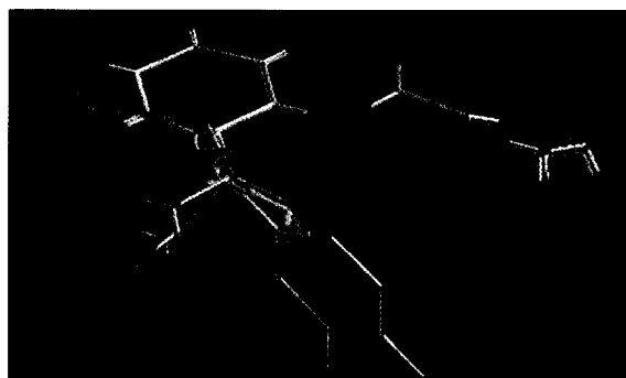
Figure 2. Steric and lipophilic contour plot for model C6 expressed as STDEV \times COEFF (contour level: -0.070 red; 0.016 green; -0.029 cyan; 0.035 yellow. Color code: see Table 7). Ligands 3 , 26 , 29 , 31 , and 32 are displayed to help interpretation.
