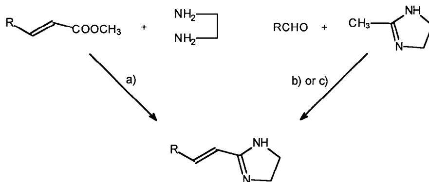
Scheme 1. Reagents and conditions: (a) \text{Al}(\text{CH}_3)_3 , toluene: compounds 4–6 , 12 , 14 , 15 , 40–42 ; (b) \Delta , butylformate: compounds 7 , 16 , 45 19 , 20 , 21 , 47 22 , 48 \Delta , ethylformate: compounds 8 , 45 10 , 11 , 13 , 24 ; (c) \Delta , toluene: compound 18 , 46 \Delta , benzene: compound 23 .
