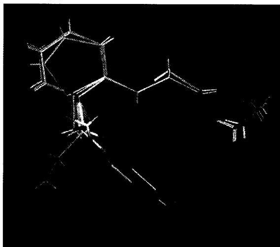
Figure 3. Steric and lipophilic contour plot for model CT5 expressed as STDEV \times COEFF (contour level: -0.070 red; 0.030 green; -0.027 cyan; 0.075 yellow. Color code: see Table 7). Ligands 5 , 22 , 32 , and 33 are displayed to help interpretation.
