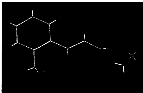
Figure 1. Lipophilic contour plot for model T3 expressed as STDEV \times COEFF (contour level: -0.015 cyan; 0.038 yellow. Color code: see Table 7). Ligands 5 and 8 are displayed to help interpretation.
