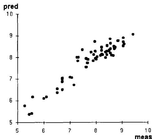
Figure 5. Plot of pK i values, predicted by general model W7 versus measured values.
